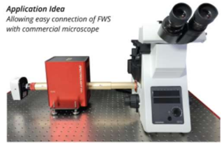
Extender accessory between a microscope and wavelength selectors and camera for imaging.
